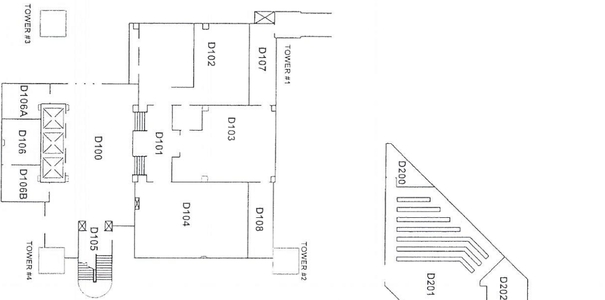
SOUTH CAMPUS "D" WING - FIRST FLOOR PLAN
